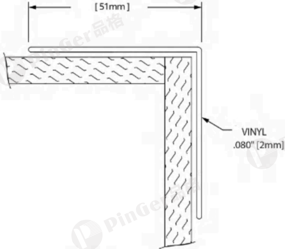
SECTION VIEW
